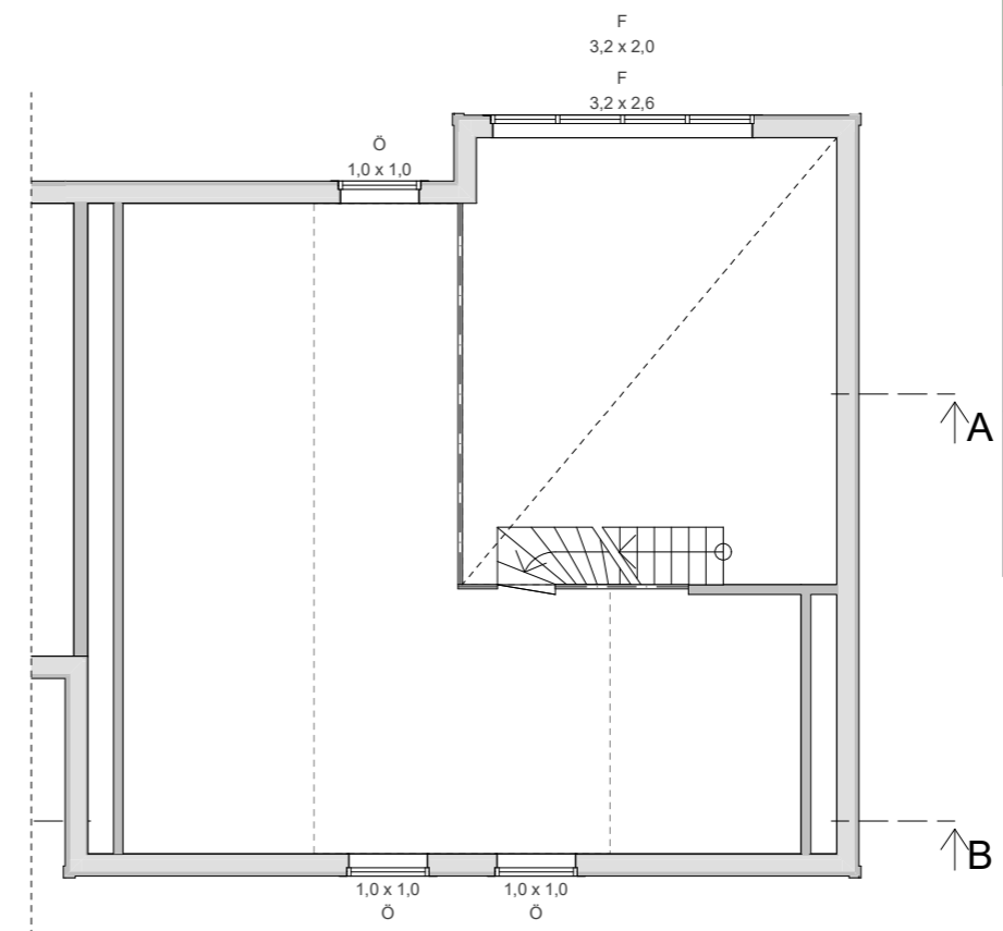
Plan Loft 1:100 BOA Loft 20,1 m 2 Golvyta Loft 46,0 m 2
