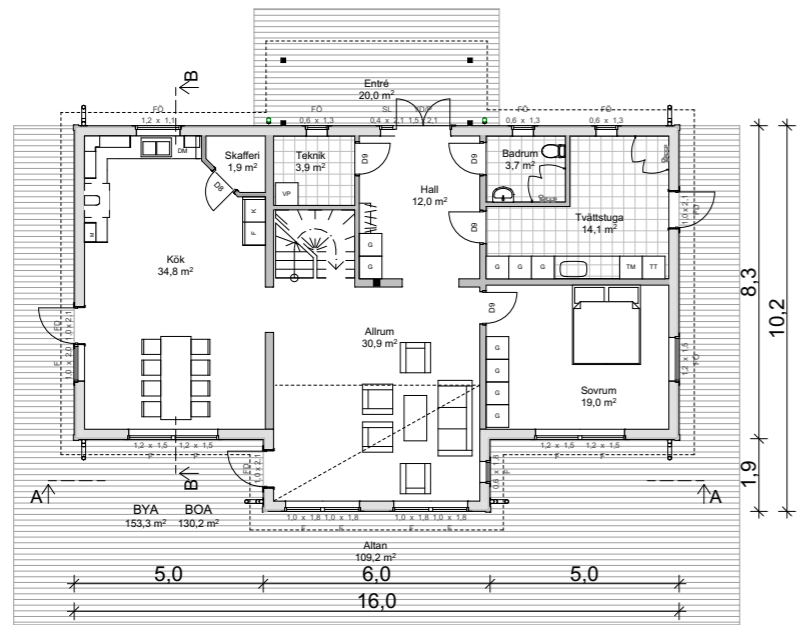
Plan 1 1:200
